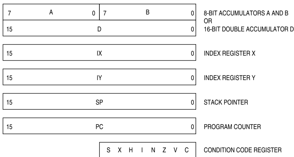
Figure 2-1. Programming Model
